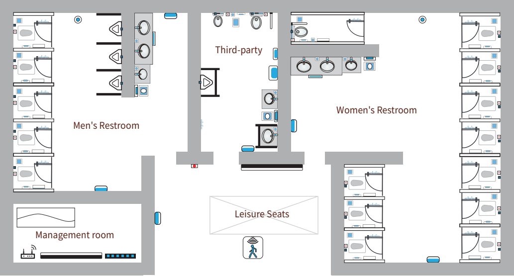
SVAVO Smart Restroom Concept Drawing
